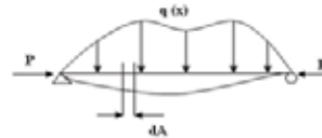
Fig 1. General loading beam-column analysis.
