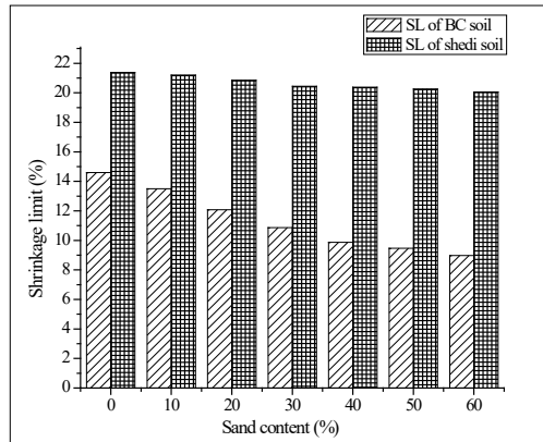
Fig.3 Percentage decreased in shrinkage limit with different content of sand
