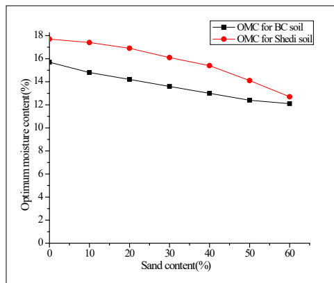
Fig.4 Variation in optimum moisture content of black cotton and shedi soil with varying sand content
