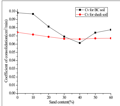
Fig. 11 Variation in coefficient of consolidation of investigating soil with varying sand content
