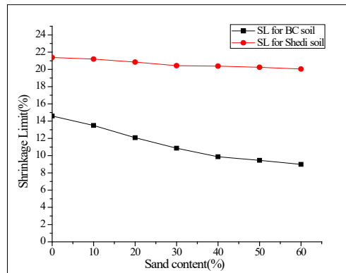
Fig. 2 Variation in shrinkage limit with different content of sand
