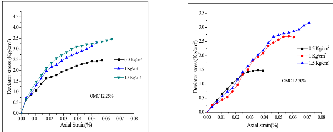
Fig. 8 Stress-strain behaviour of BC and shedi soil with 60% of sand content
