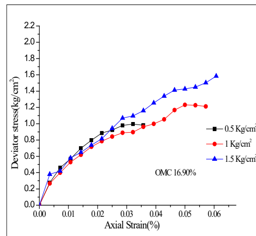
Fig. 7 Stress-strain behaviour of BC and shedi soil with 10% of sand content
