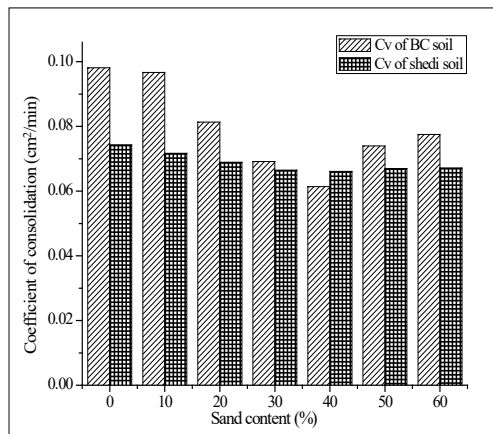
Fig. 12 Percentage decreased in coefficient of consolidation of investigating soil with varying sand content
