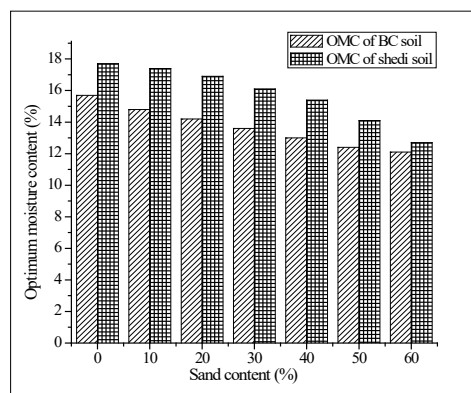
Fig.5 Percentage decreased in optimum moisture content of investigating soils with varying sand content
