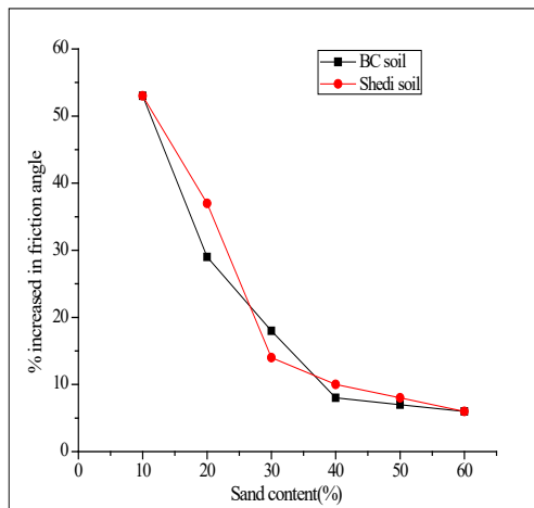
Fig. 10 Percentage increased in friction angle of investigating soil with varying sand content
