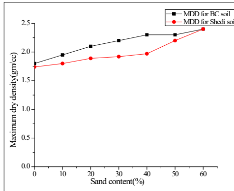
Fig.6 Variation in maximum dry density of black cotton and shedi soil with varying sand content
