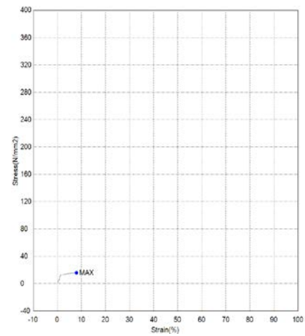
Fig. 16 Force displacement and stress strain curve For 16% mortar
