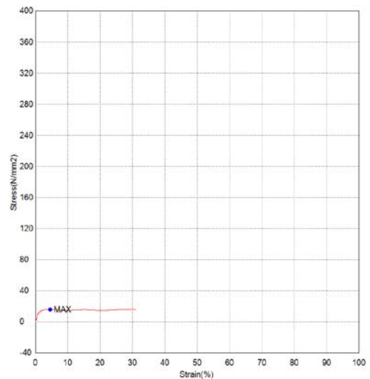
Fig. 8 Force vs displacement and stress vs strain curve For 0% mortar
