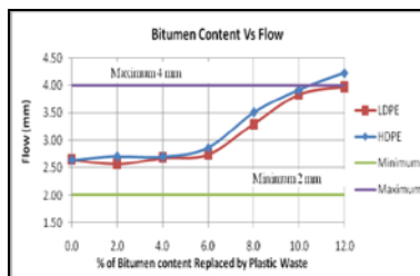
Fig.7 Bitumen Content Vs Flow
