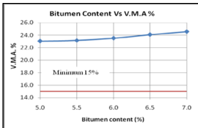
Fig. 2 Bitumen content Vs V.M.A%
