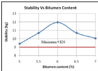
Fig.1 Stability Vs Bitumen Content
