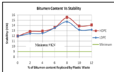
Fig.6 Bitumen Content Vs Stability
