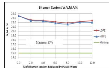
Fig.8 Bitumen Content Vs V.M.A. %
