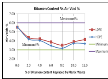
Fig.10 Bitumen Content Vs Air Void %
