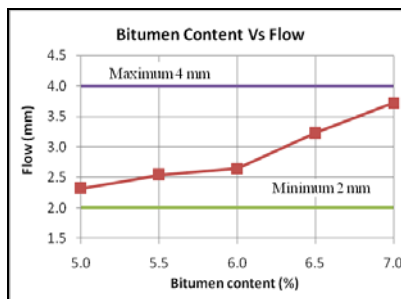
Fig. 5 Bitumen Content Vs Flow
