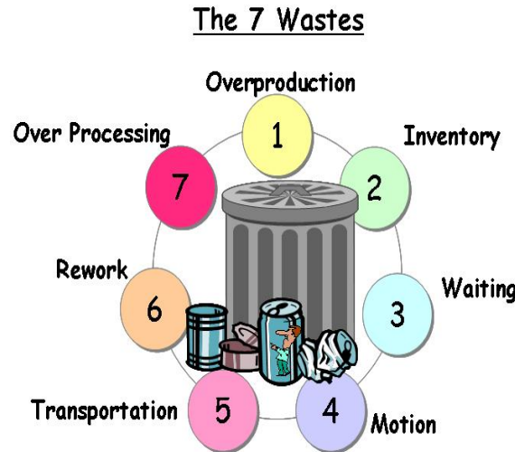
Fig.2 The 7 wastes
